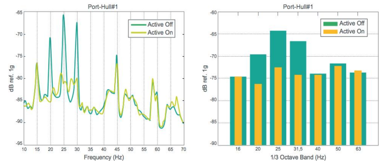
Active Vibration Control Test Results
